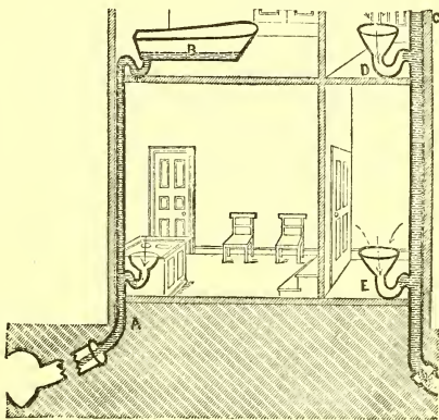
FIG. 19.—Traps being siphoned out.
